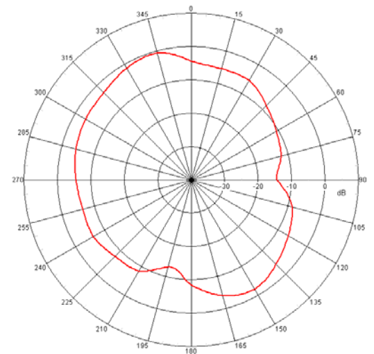
XZ-plane @2450MHz Total
