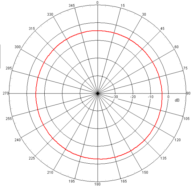
XY-plane @868MHz — Total
