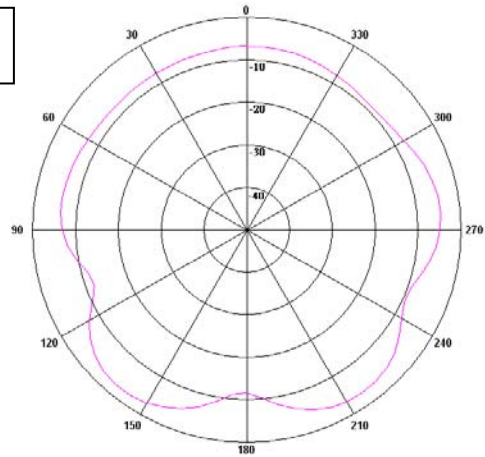
XY cut @490MHz — Total
