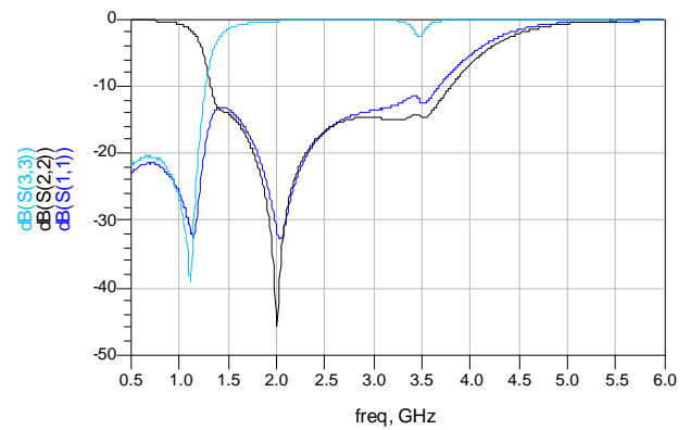
Return Loss
