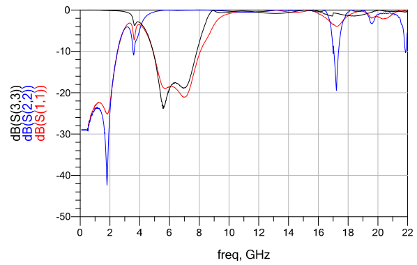
Return Loss
