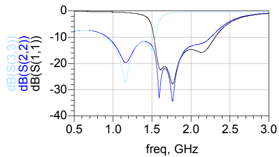
Return Loss
